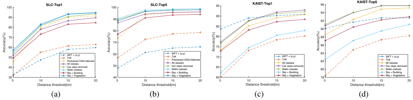
Fig. 5. Localization accuracies. (a) and (b) represent the results for SLC Urban dataset while (c) and (d) represent the results for KAIST dataset. The x-axis represents the distance threshold and the y-axis represents the accuracy. Non-CASENet results are shown using dashed lines. No weighting of features are applied. Note for KAIST, the pretrained VGG-NetVLAD performances are very low (and even with retraining), thus we do not include them here. Note CASENet is not retrained either.
